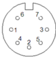
Figure 2: Pin assignment of handswitch socket; pin alignment according to DIN 45329
